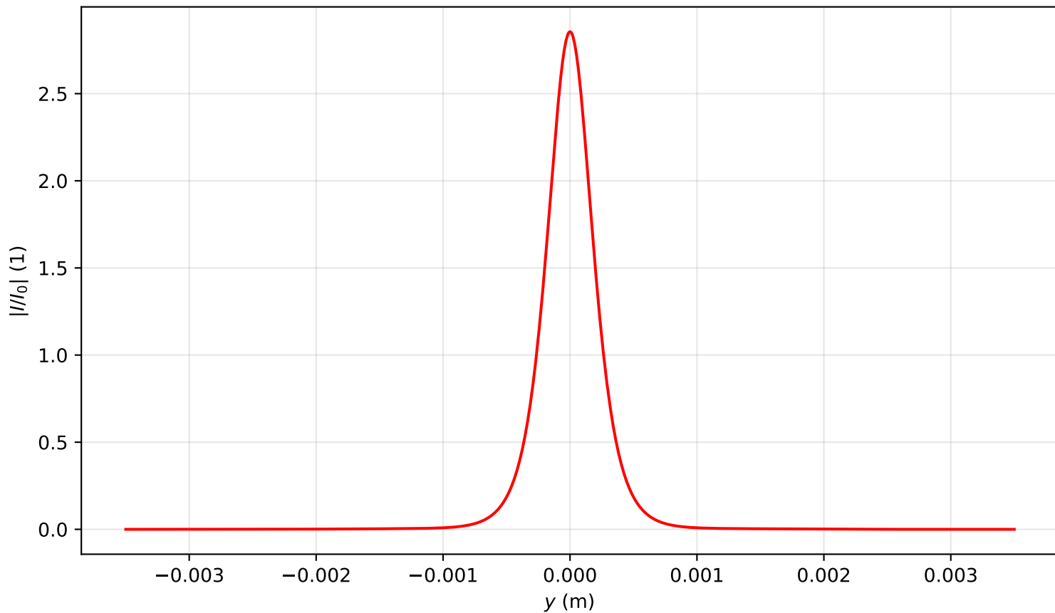
Intensity profile I(x=0, y, z=3.344)/I_0 , P_{in}=1.0P_{cr} , artificial time
